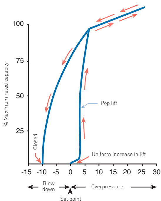
FIGURE 6 TYPICAL FLOW CURVE - CONTOURED TRIM DESIGN (JLT)
