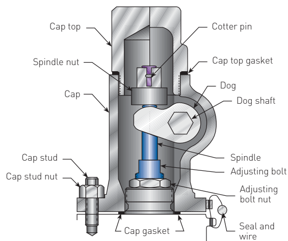
Packed lifting lever Type D
