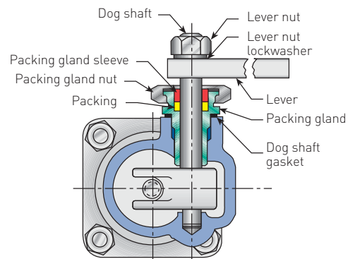
Packed lifting lever Type D
