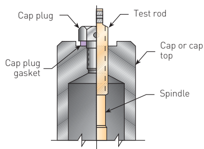
Cap and test rod
