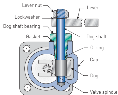
Packed lifting lever Type D
