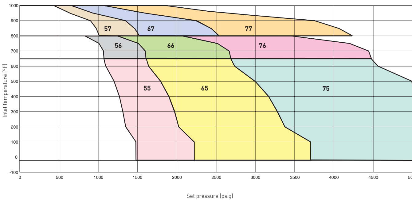
PRESSURE/TEMPERATURE LIMIT CHART - ANSI CLASS 900, CLASS 1500, CLASS 2500 F Orifice, 0.307 sq.in. [198 sq.mm] API effective area
