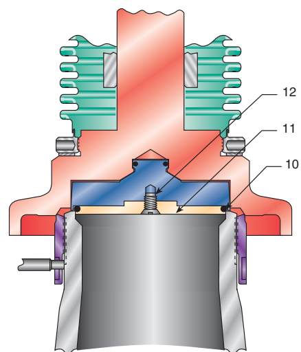
SERIES JBS-E (with O-ring seat)
