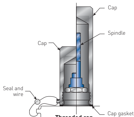
Threaded cap
