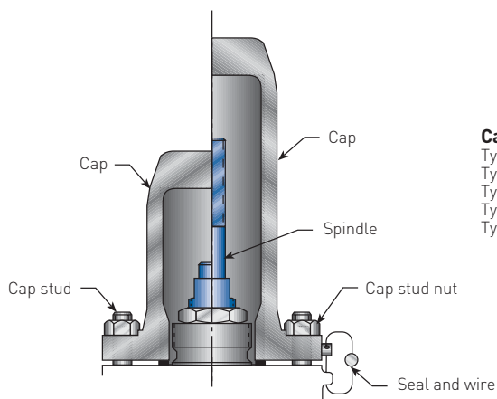
Bolted cap
