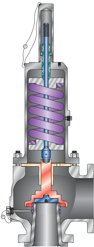
SERIES JOS-E (with metal-to-metal seat)
