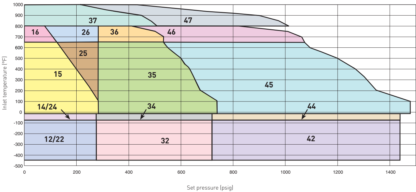
PRESSURE/TEMPERATURE LIMIT CHART - TO ANSI CLASS 600 D Orifice, 0.110 sq.in. [71 sq.mm] API effective area
