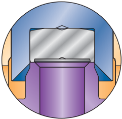
Metal-to-metal seat
