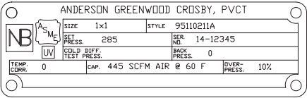
Sample nameplate (for illustrative purposes only)
