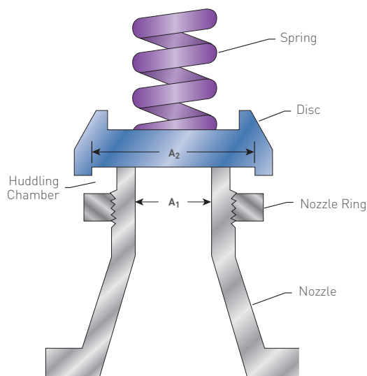
FIGURE 4-5 Generic Direct Spring PRV Trim
