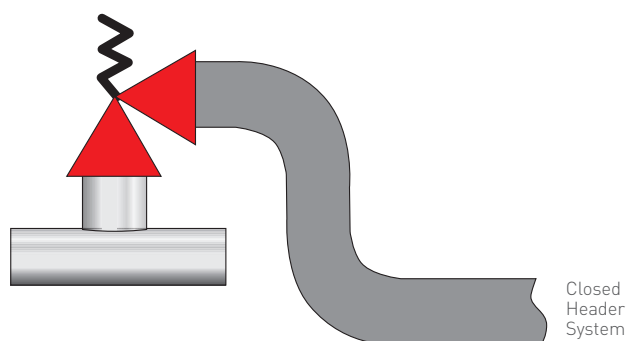
FIGURE 4-20 Closed Header System Discharge Piping
