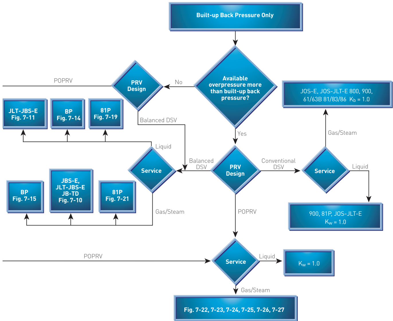
Valve Selection Recommendations for Built-up Back Pressure Installations (No Superimposed Back Pressure)
