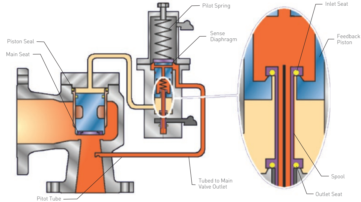
FIGURE 4-33 Modulating Action Pilot Operated PRV (open and in full lift)
