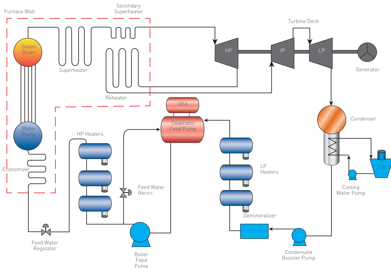
FIGURE 5-2 Closed Simple Rankine Steam Cycle
